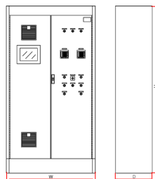
L x W x H 50 x 22 x 76 in Protection NEMA-1
