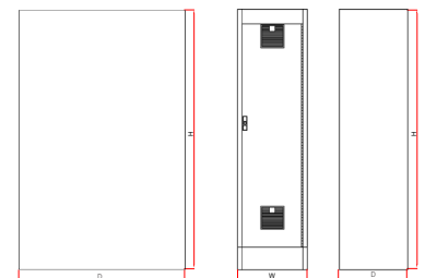
L x W x H 25 x 22 x 76 in Protection NEMA-1
